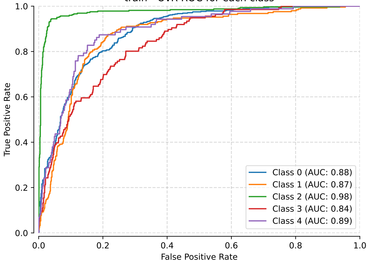
train - OvR ROC for each class
