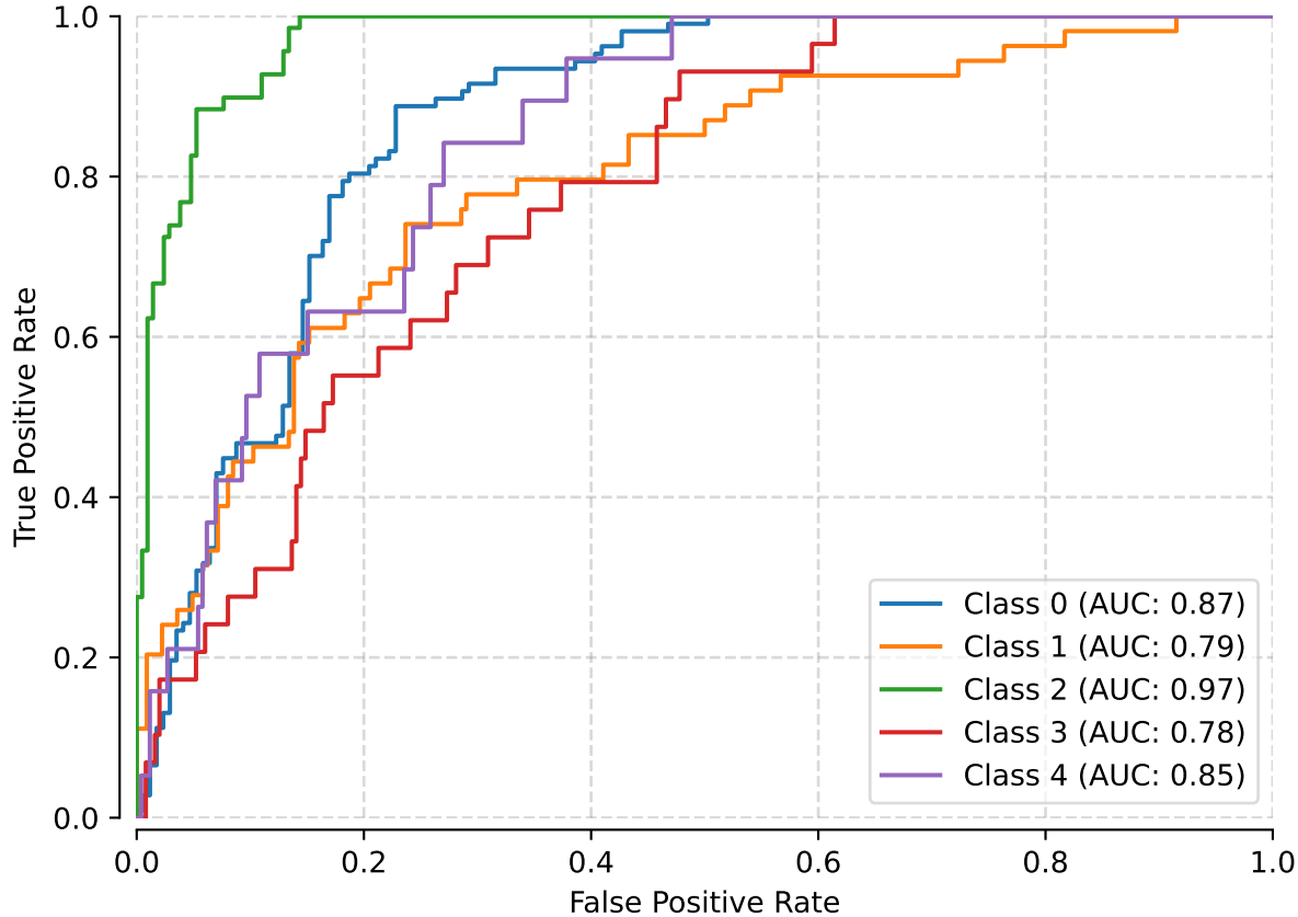
test - OvR ROC for each class
