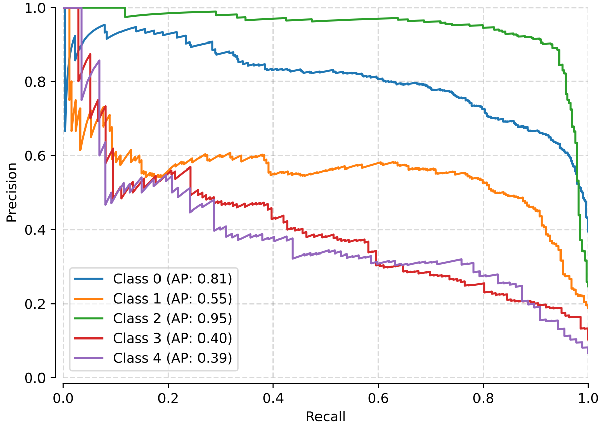
train - Precision-Recall curve for each class
