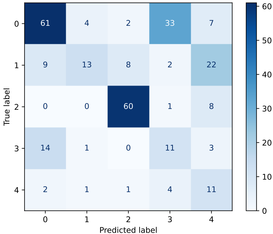
Confusion Matrix - test
