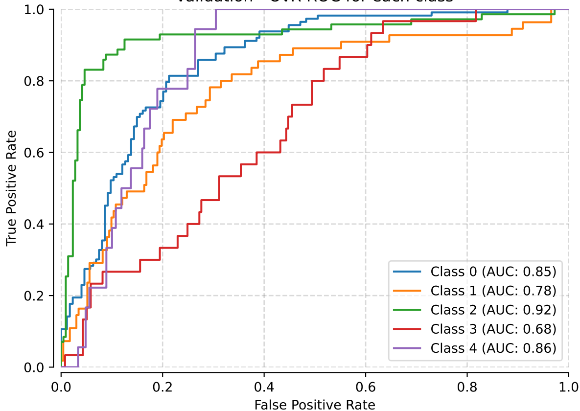
validation - OvR ROC for each class
