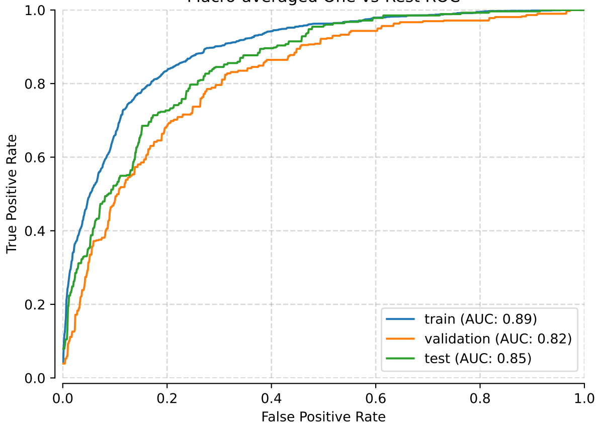
Macro-averaged One-vs-Rest ROC
