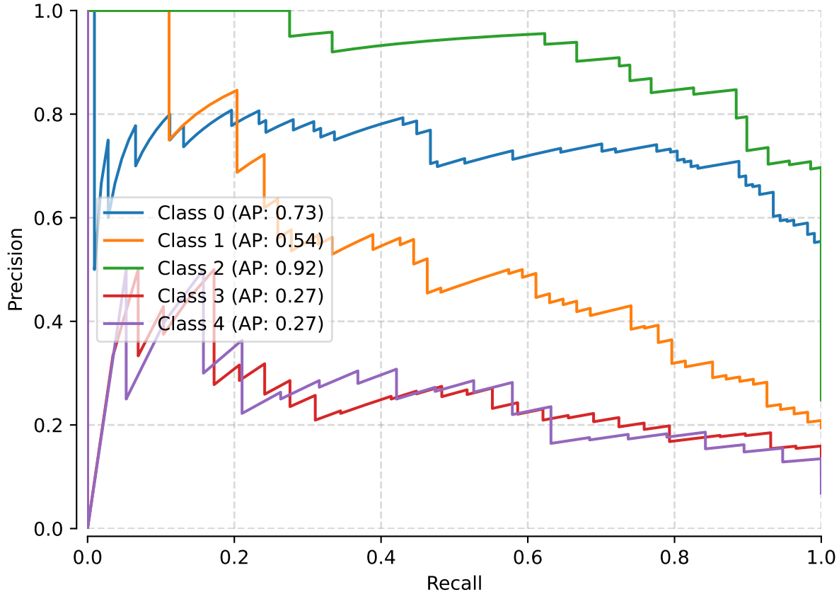
test - Precision-Recall curve for each class
