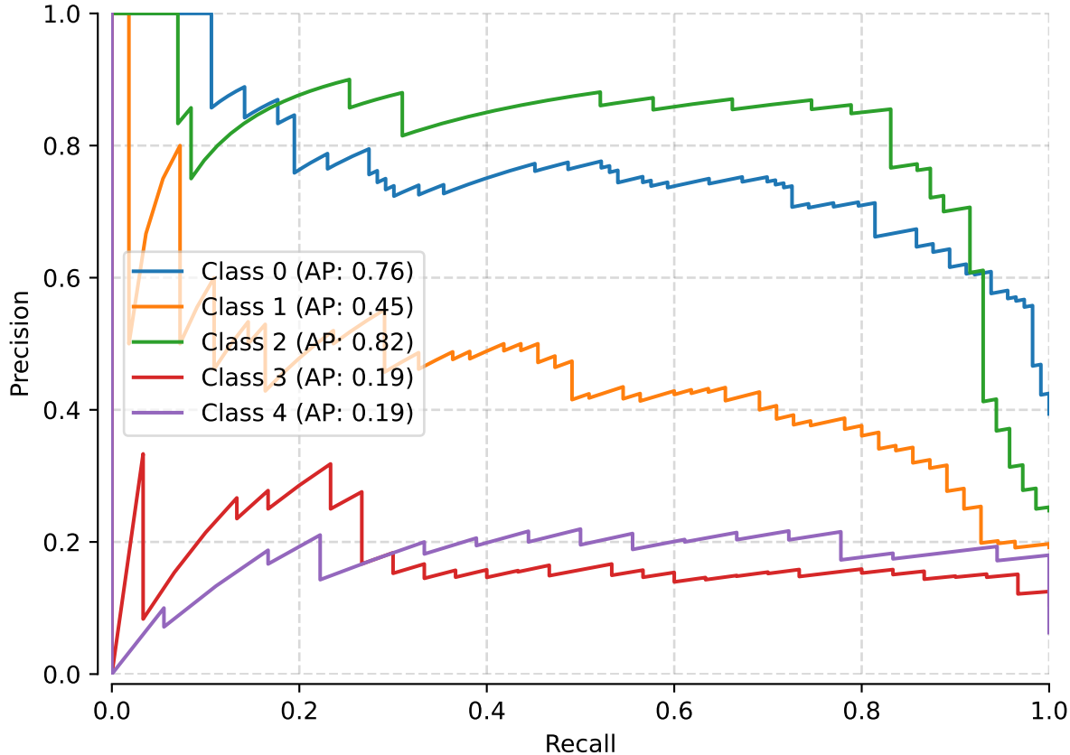
validation - Precision-Recall curve for each class
