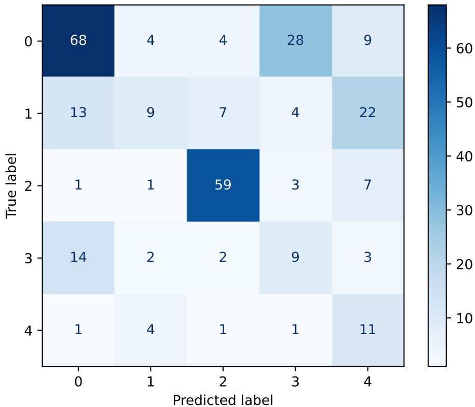
Confusion Matrix - validation
