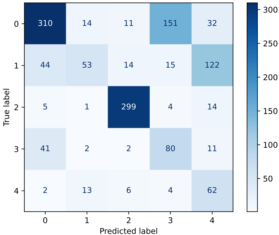
Confusion Matrix - train
